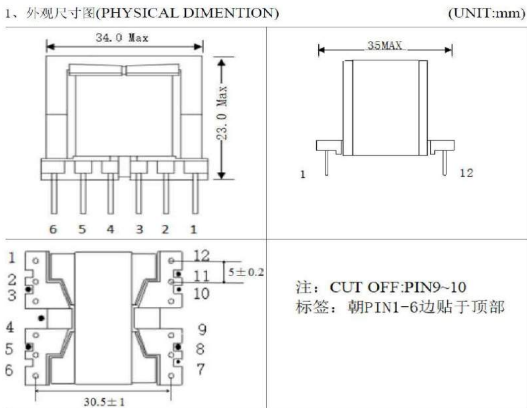
Illustration 4a- Specification for transformer
