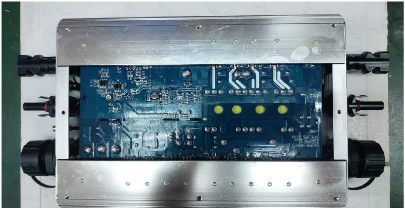
Photo 14- Internal view of model WVC-600, WVC-700
