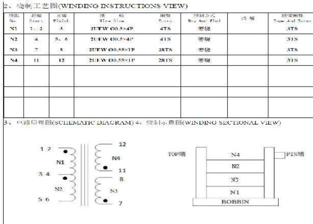
Illustration 5a- Specification for transformer
