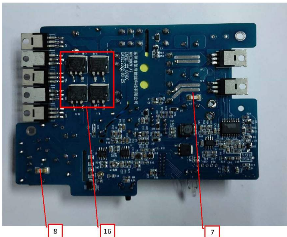
Photo 8- PCB board view (Soldered side), model WVC-300, WVC-350
