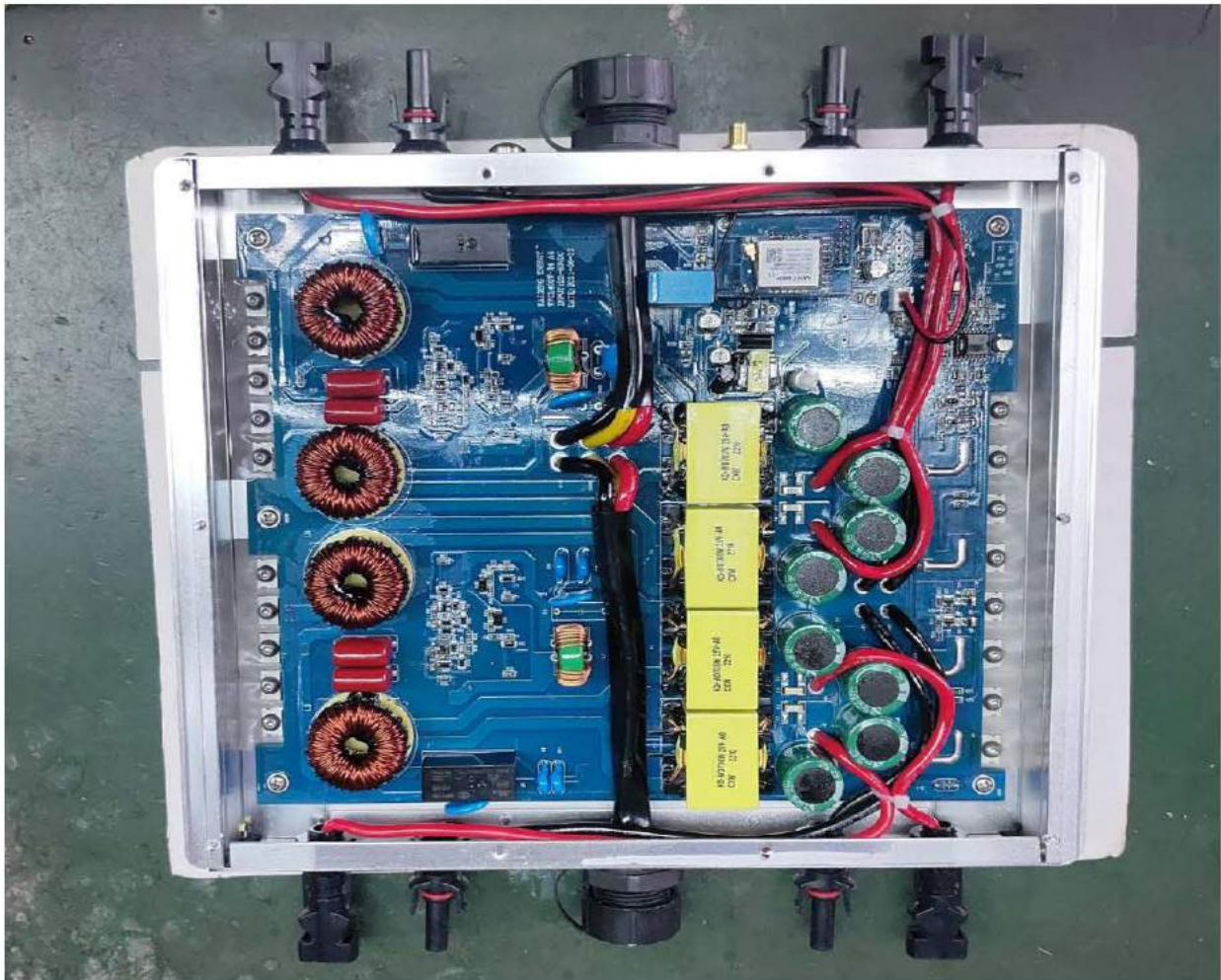
Photo 18- Internal view of model WVC-1200, WVC-1400
