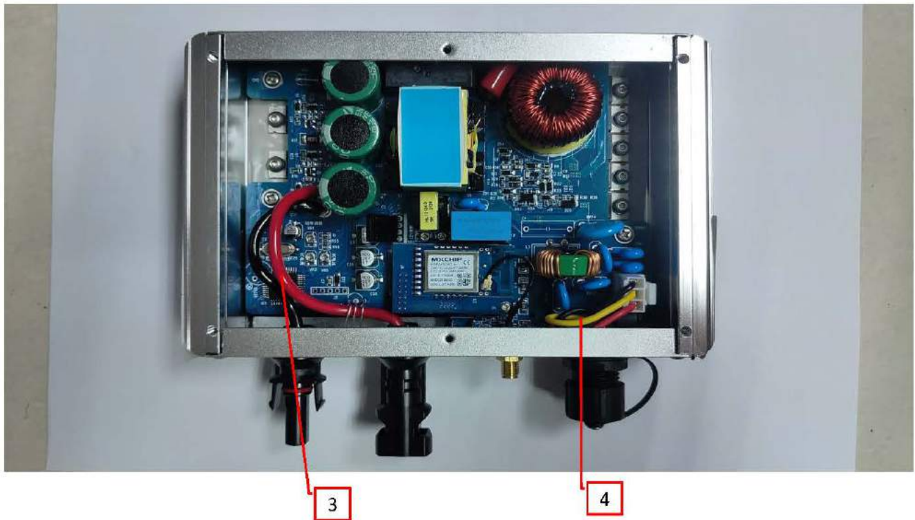
Photo 5 - Internal view of the unit (before Pouring sealant),model WVC-300, WVC-350
