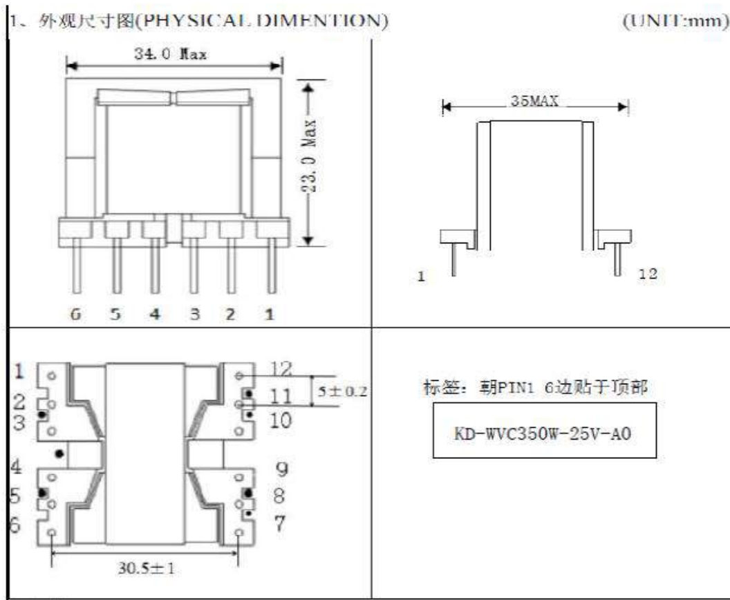
Illustration 5a- Specification for transformer
