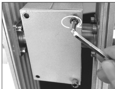
8. Fix the pole cover by 4pcs M4*8 screw
