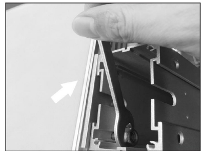
6. Tighten the nut with a wrench
