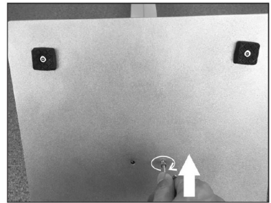
3. Fix the bottom pole onto the base by 4pcs M4*20 screw
