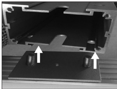
4. Insert the lamp holder screw into the pole
